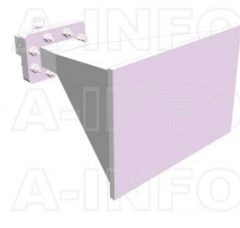
LB-187-15-C-NFSPO Standard Gain Horn Antenna 3.95-5.85GHz 15dB Gain N Type Female
