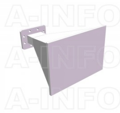
LB-187-15-ASPO Standard Gain Horn Antenna 3.95-5.85GHz 15dB Gain Rectangular Waveguide Interface
