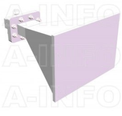
LB-187-15-C-SFSPO Standard Gain Horn Antenna 3.95-5.85GHz 15dB Gain SMA Female
